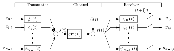
Figure 2.3: Base-band OFDM system model.
